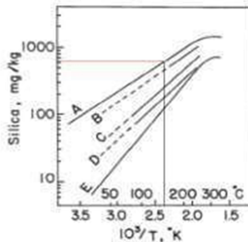
Figure 7: Silica content and saturation teperature [9]
