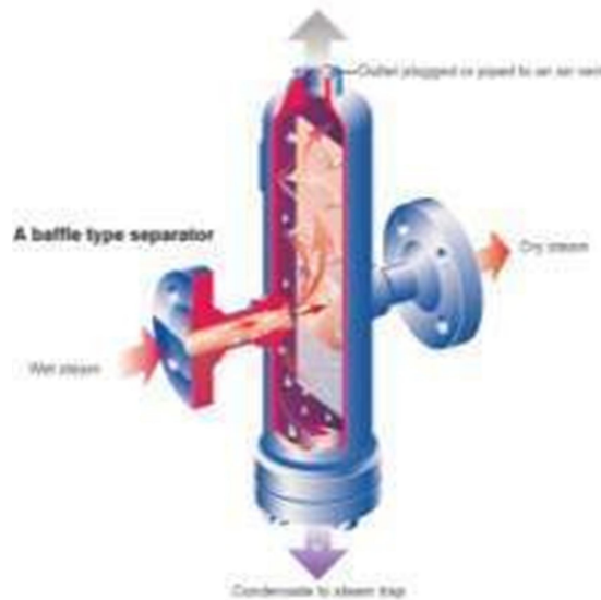
Figure 4: Baffle Type Separator
