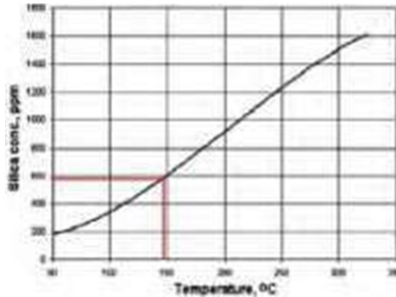
Figure 8: Silica content and saturation temperature.
