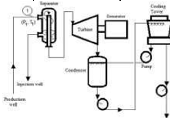
Figure 3: Separated Steam Cycle System [4]
