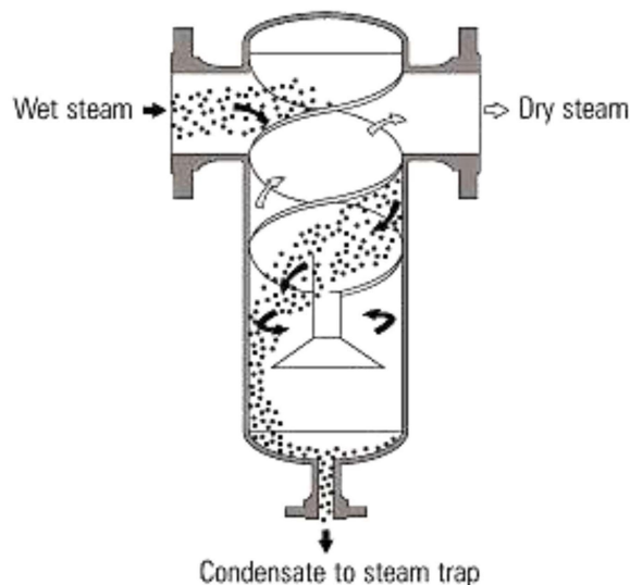
Figure 6: Cyclone type separator
