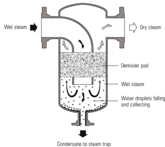
Figure 5: Coalescence Type Separator
