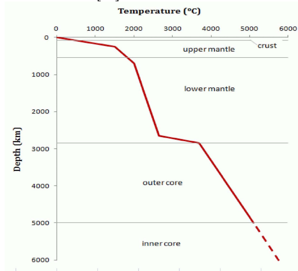
Figure 1: Geothermal gradient. Temperature inside the earth gradually increases with depth due to the interior heat flux. The average gradient in the earth crust is approximately 25°C/km.[5]
