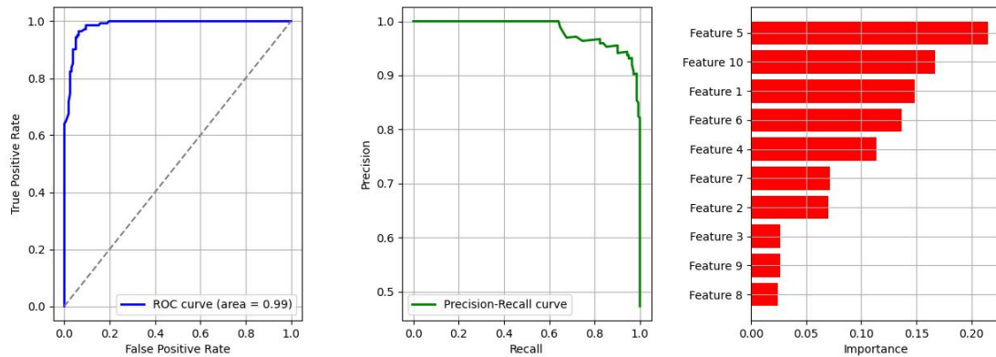
Figure 3: Model Performance Analysis
