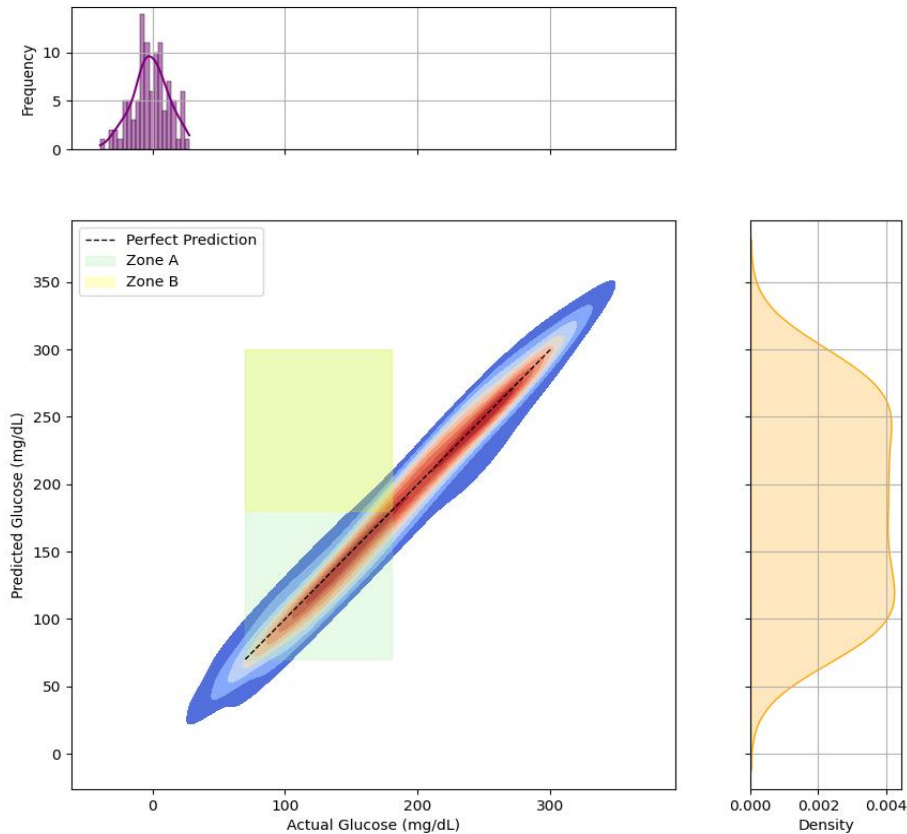
Figure 5: Prediction Error Distribution Analysis
