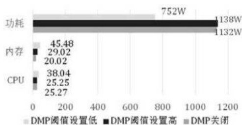
Figure 2: Energy saving effect of dynamic resource management
