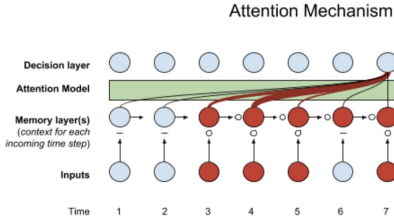
Figure 1: Attention Mechanism
